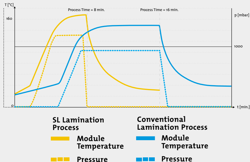
Diagram of SL Process versus Conventional Process
